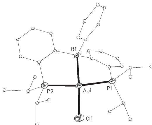
Figure 1. Molecular structure (thermal ellipsoids set at 50% probability) of complex 2a in the solid state. Hydrogen atoms are omitted for clarity.
