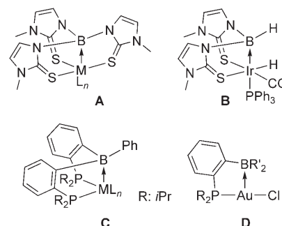
Scheme 1. Structurally characterized complexes featuring M \rightarrow BR_3 interactions.
