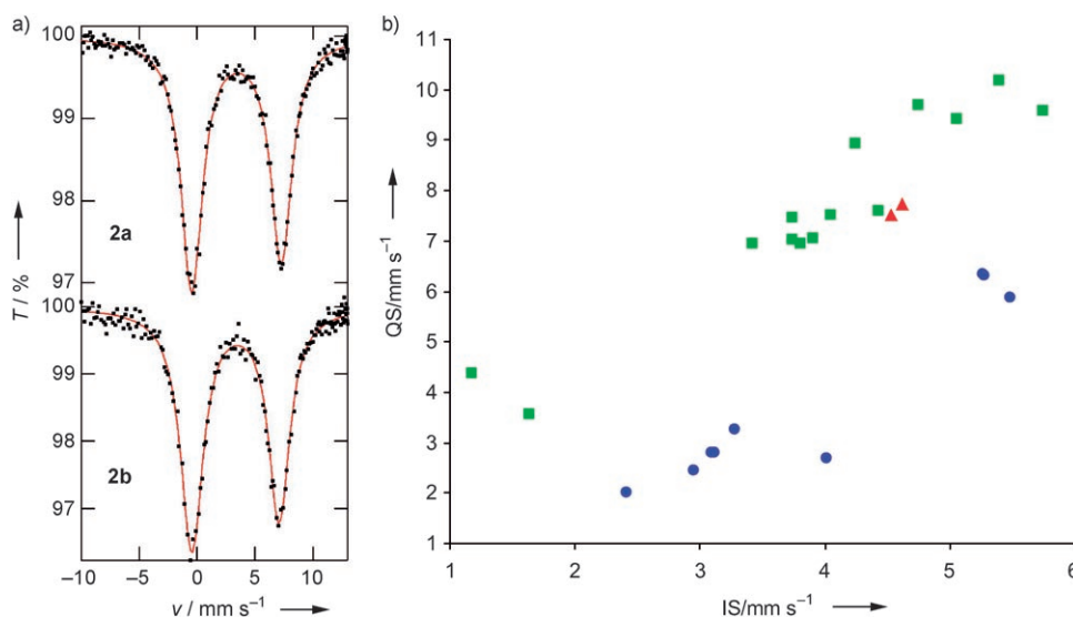
Figure 3. a) 197 Au Mössbauer spectra for complexes 2a,b at 12 K. T = Relative transmission, v = Doppler velocity. b) QS/IS correlation for complexes 2a,b (red triangles) and representative phosphane complexes of gold(I) (green squares) and gold(III) (blue circles). IS values are given relative to gold metal.
