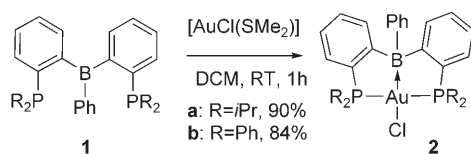
Scheme 3. Coordination of the ambiphilic diphosphanylborane ligands 1a,b to AuCl.
