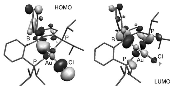
Figure 2. Frontier orbitals for complex 2a* . Hydrogen atoms are omitted for clarity.
